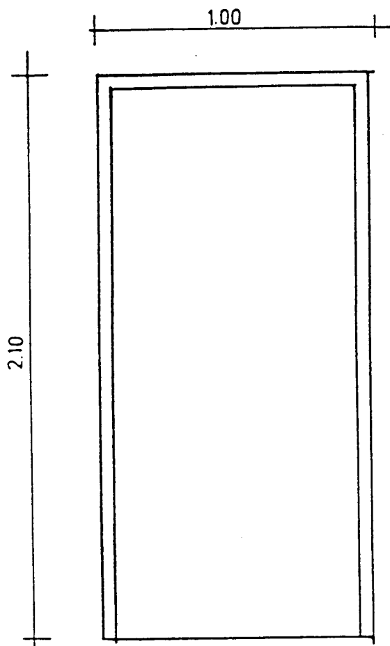
DETAIL OF DOOR FRAM SCALE 1/20
